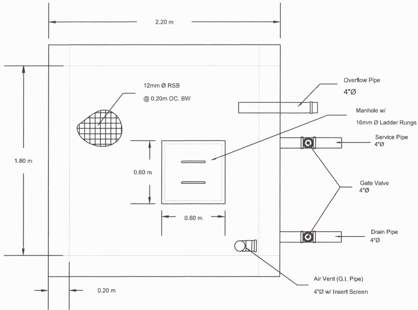
TOP VIEW OF SPRING BOX
