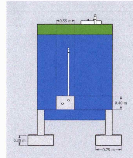
RIGHT VIEW
