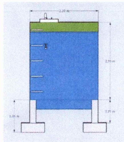
LEFT VIEW
