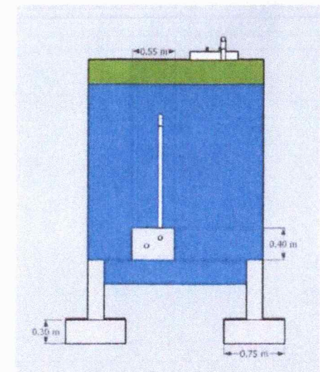
RIGHT VIEW
